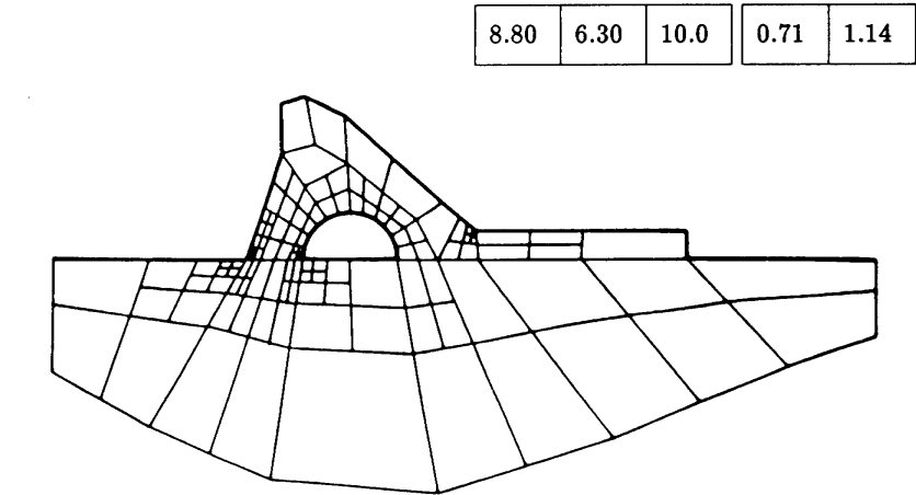
Malla 4 (914 GDL)
