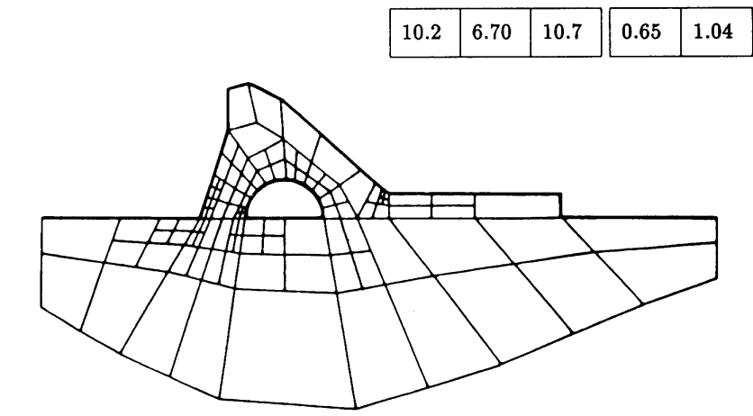
Malla 3 (834 GDL)
