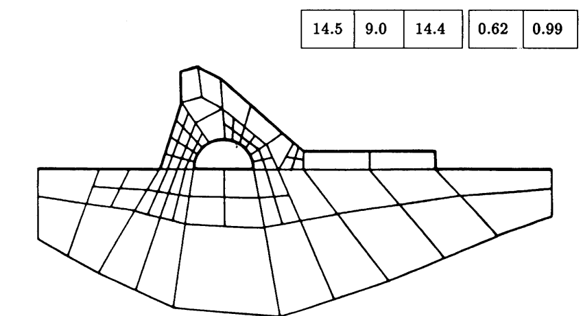
Malla 2 (610 GDL)
